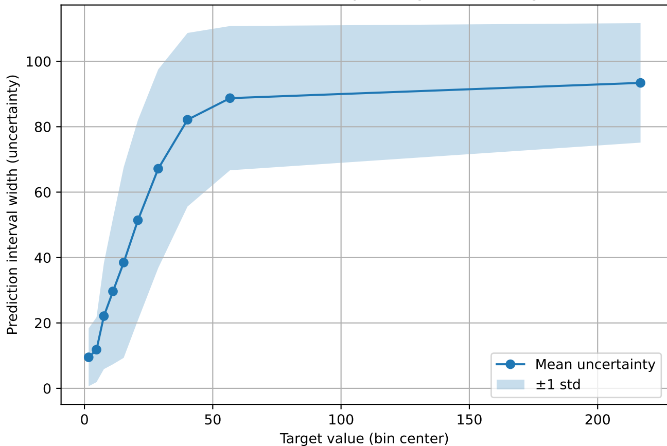
BPIC20ID: Uncertainty vs Target Value Range
